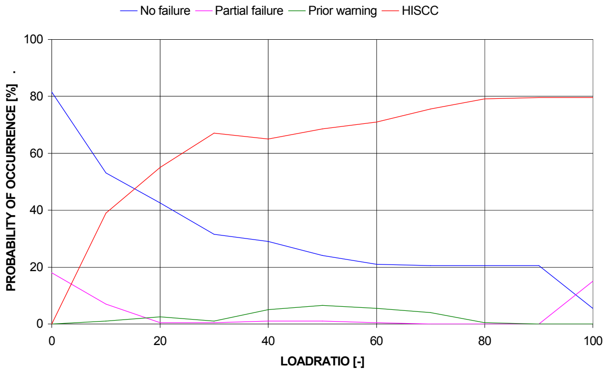
Figure 7 Influence of Load Ratio on the Probability of HISCC - Failure
