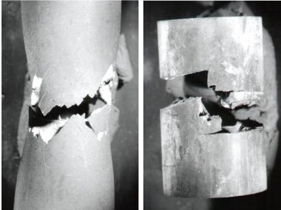
Figure 1 Left: Rupture (ductile fracture) Right: Stress Corrosion Cracking (Hydrogen induced)
