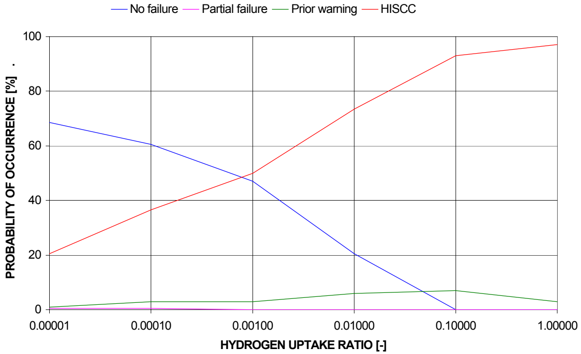
Figure 6 Influence of Hydrogen Uptake Ratio on Probability of HISCC - Failure
