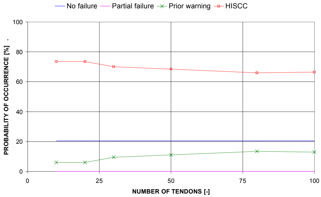
Figure 10 Degree of Redundancy against HISCC - Failure by Number of Individual Tendons/Wires
