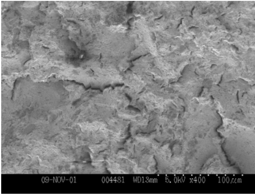
Figure 8 Hydrogen induced Cracks in Steel
