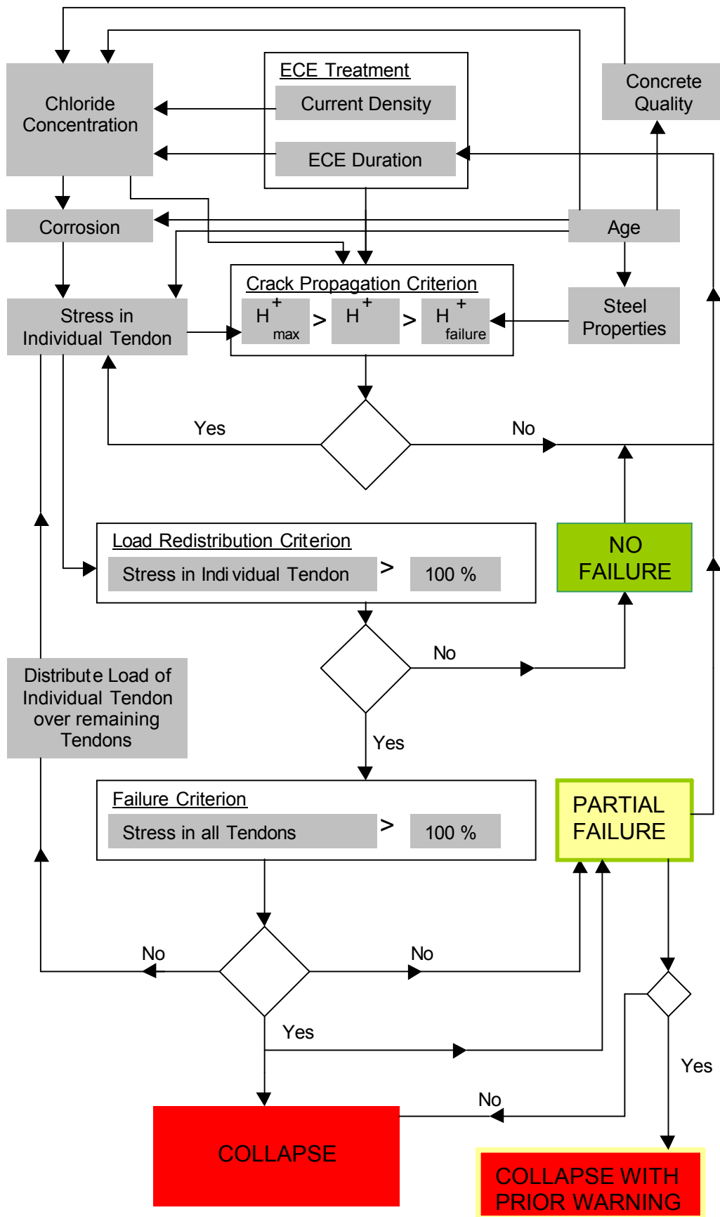
Figure 3 Fault tree analysis of parameters leading to crack propagation and HISCC failure
