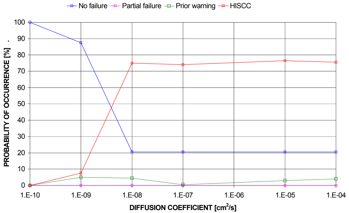
Figure 9 Influence of Hydrogen Diffusion Coefficient on Probability of HISCC - Failure
