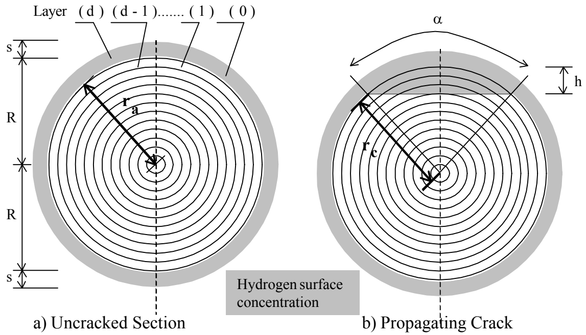
Figure 4 Geometry of Prestressed Bar with Crack Propagation
